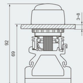
Cover mounting
